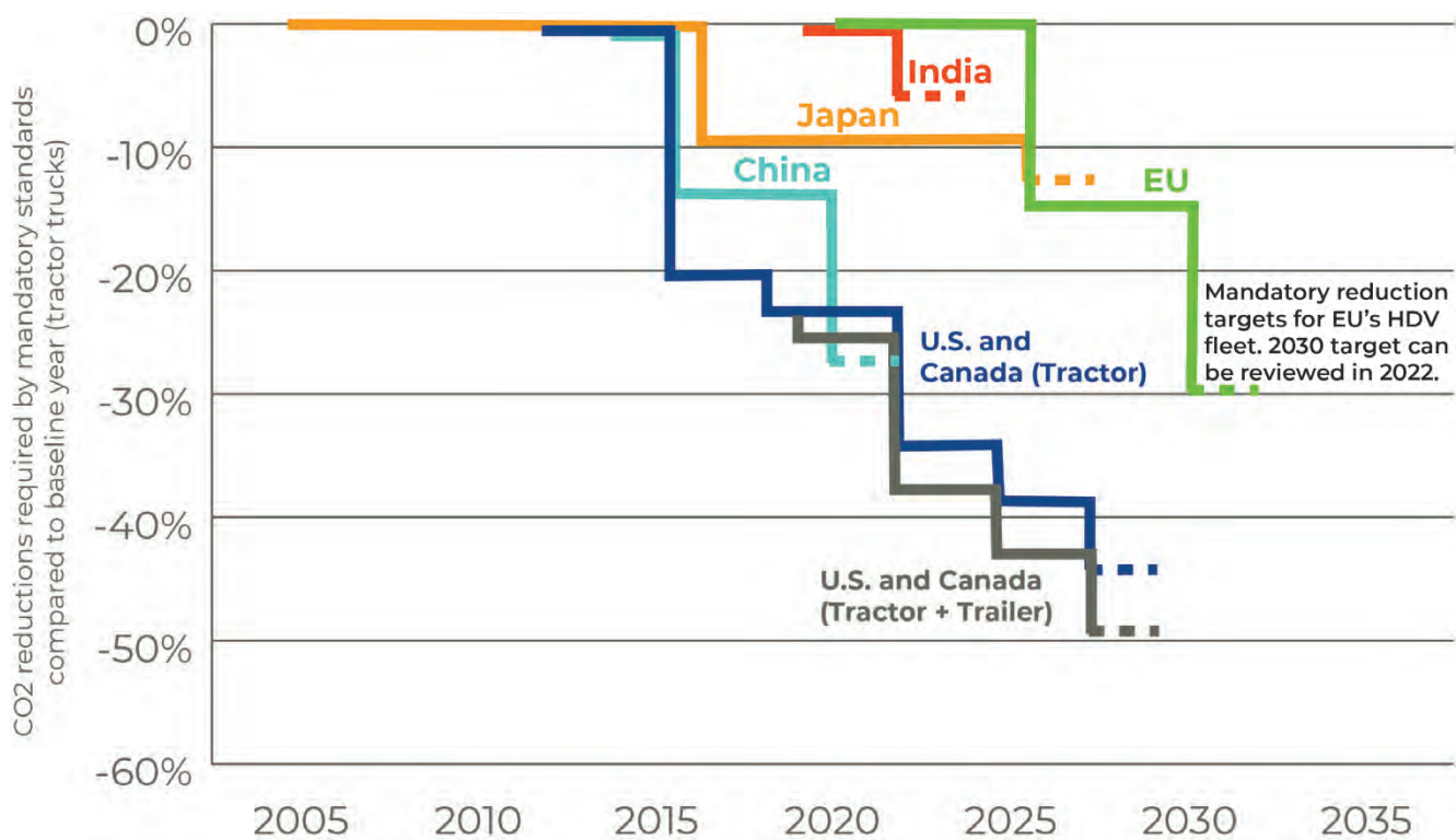
Figure 5-1. National and regional MHDV fuel economy standard targets
