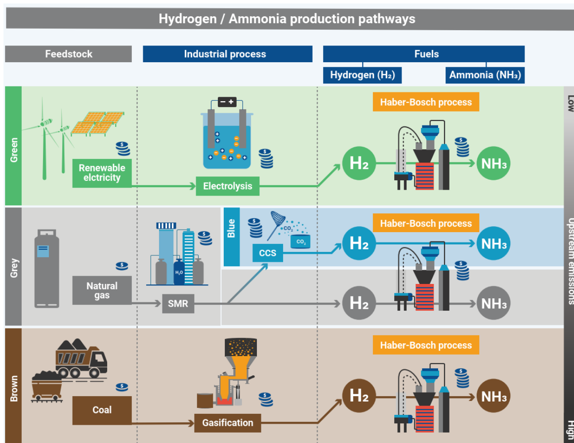
Figure 2 Hydrogen and ammonia production routes
